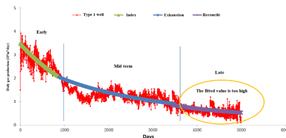
Figure 6. The law of late production decline of tight gas wells
