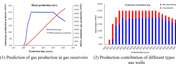
Figure 9. Block production and production contribution characteristics of different gas wells
