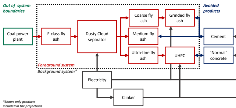
Figure 2 System scope of the innovative technology
