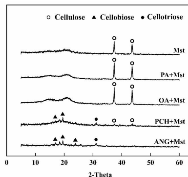
Fig. 7. XRD patterns of the straw in each treatment after seven days of incubation.
