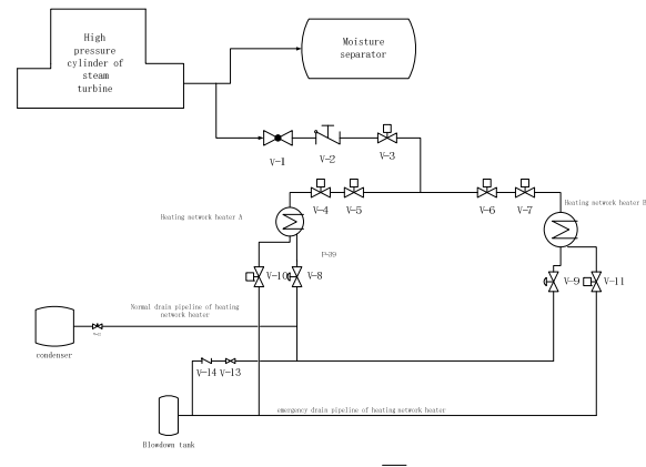
Fig. 1 flow chart of heating network heating system
