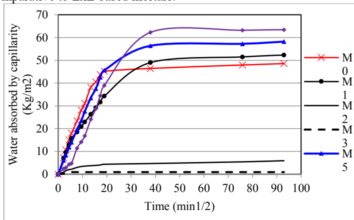
Fig. 4: Water absorbed by capillary of all earth based-mortars
