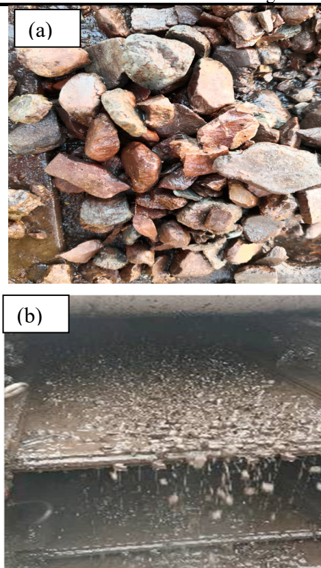
Fig. 9. Heavy pulp belt out of block(a) and thick slurry brings out lumps(b)
