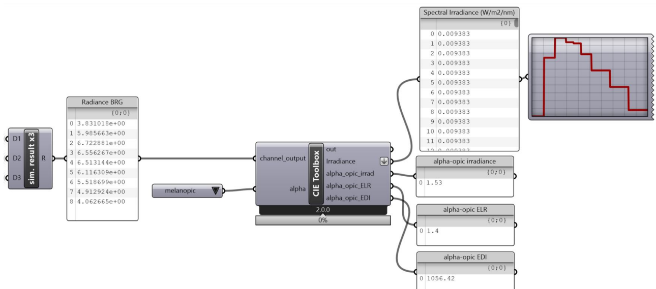
Figure 3: Implementation of the CIE toolbox in a Grasshopper component.
