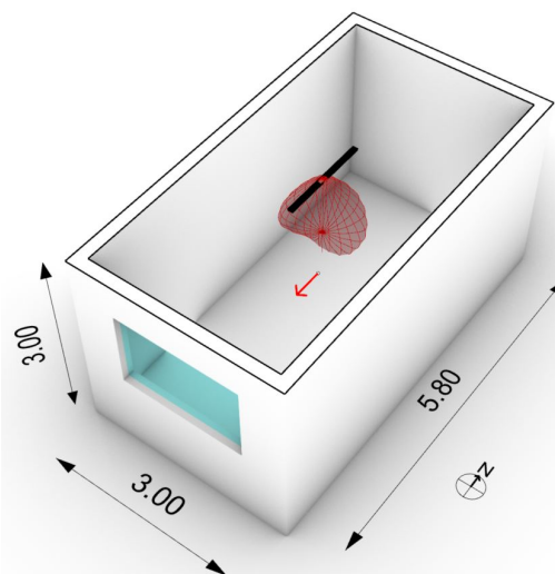
Figure 7: Simple room model. The red arrow indicates the grid point and direction. The red web under the luminaire indicates the luminous intensity plot.
