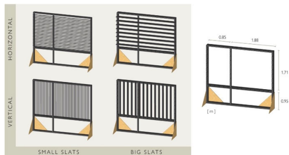
Figure 4: Left: Visualizes the frame with the four solar shadings. Right: the measurements of the frame.
