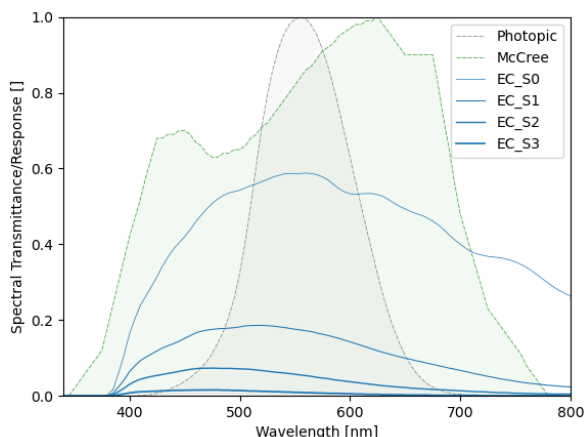
Figure 2: Spectral transmittance of different states of EC and the response function for photopic and McCree
