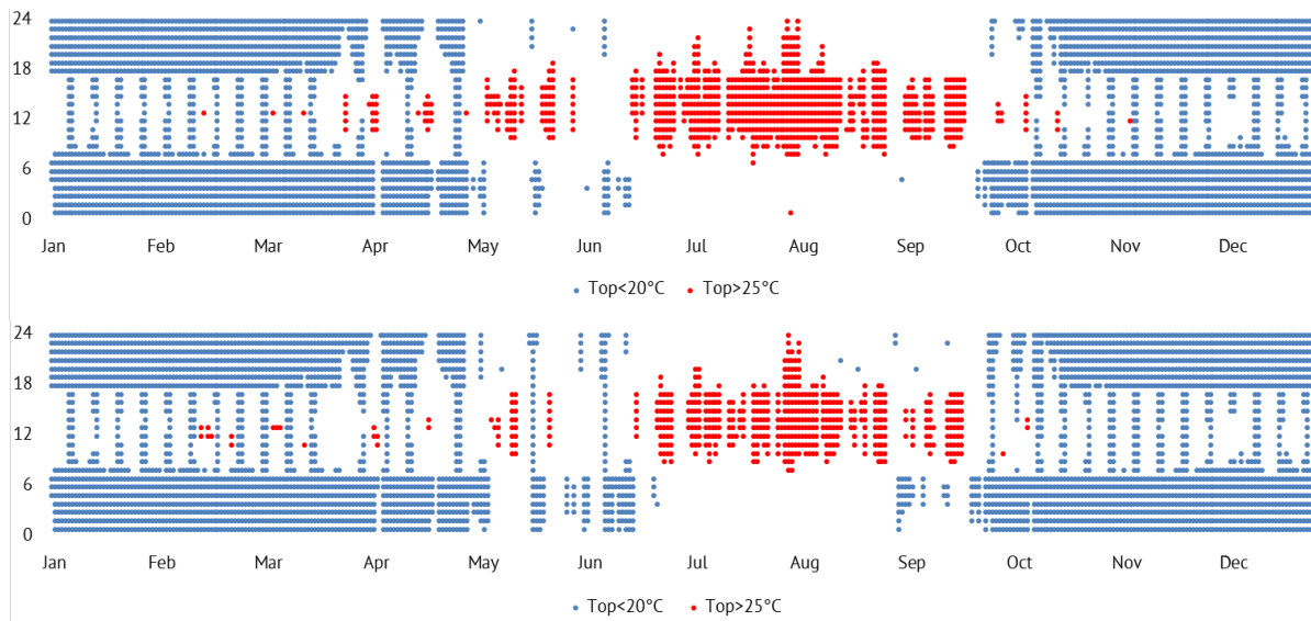
Figure A-2. Hourly simulated operative temperature ( T_{op} ) inside the office room influenced by different control strategies: a) Radiation based control (CtrlRad), b) Penalty based control (CtrlPen)
