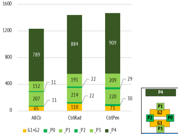
Figure 6: Total annual electricity demand kWh for supplemental lighting for occupants (G1+G2), potted plants (P0-P3), and green wall (P4) under three different control conditions Table 8 shows the total supplemental electrical demand for lighting and its equivalent primary electricity and CO 2 emission under three different control conditions.
