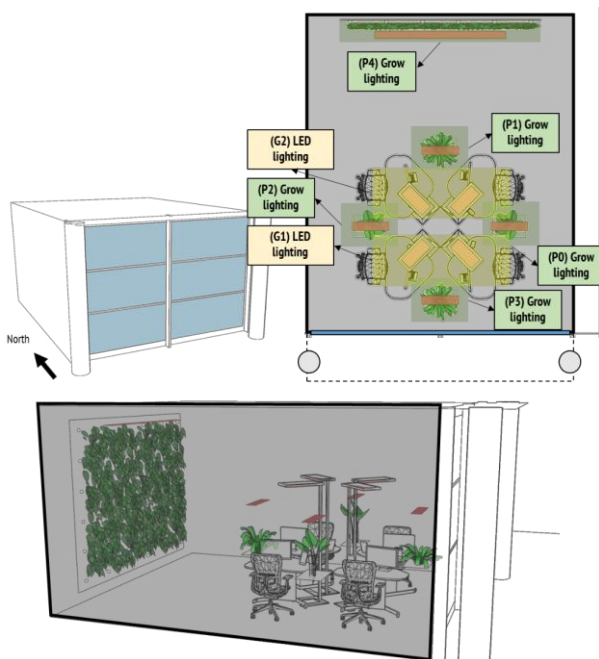
Figure 1: Visual representation of the prototypical room; plan layout of the workstations, luminaires (G1 and G2), and the indoor plants and the grow lightings (P0-4)
