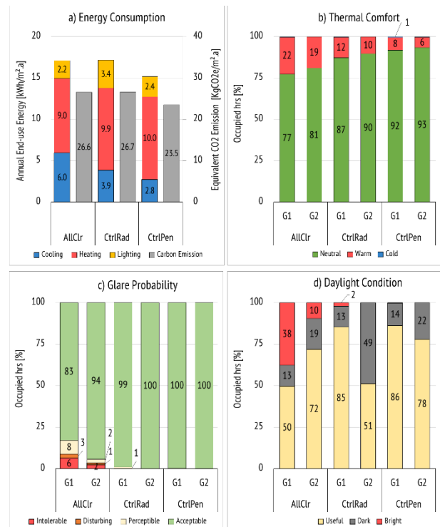
Figure 3: overall performance of the room with a switchable EC under three different control conditions (AllClr, CtrlRad, and CtrlPen): a) electricity consumption, b) thermal comfort, c) glare probability, and d) useful daylight
