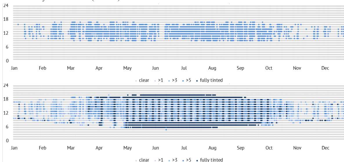
Figure A-1. a) Hourly states of the EC under Radiation based control (CtrlRad), b) Hourly states of the EC under Penalty based control (CtrlPen) as it was applied in simulations
