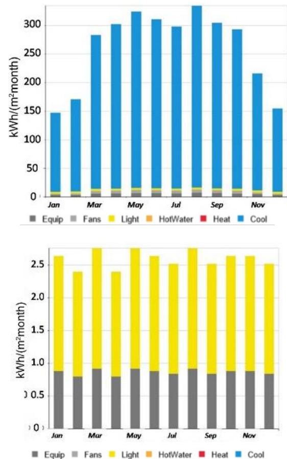
Figure 6: EUI results for base case (top), EUI results after completion of eight steps (bottom)
