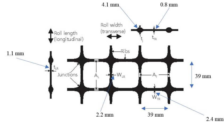
Fig. 2. The Biaxial geogrid details
