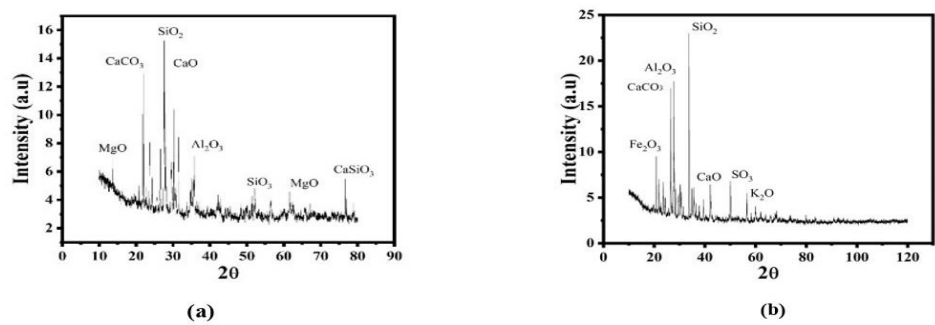
Figure 2. X-RD results of virgin aggregate(a) and RAP(b)
