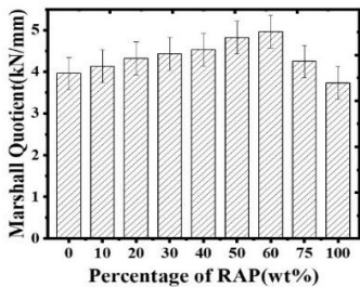
Figure 5. Marshall quotient of RAP-8%SDA modified BC mix
