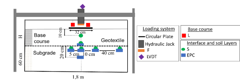
Figure 2: Instrumentation system
