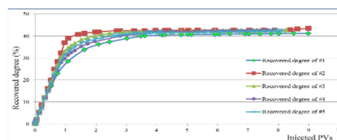
Figure 6. Comparison of the recovered degrees of the physical models
