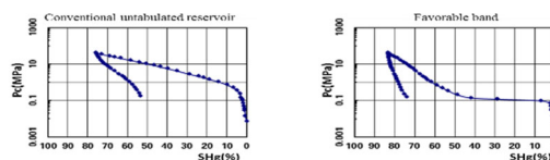
Figure 2. Comparison of the mercury intrusion curves of the conventional untabulated reservoir and favorable band
