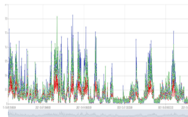
Fig. 1 Acceleration data sampling of main bearing rear end cover
