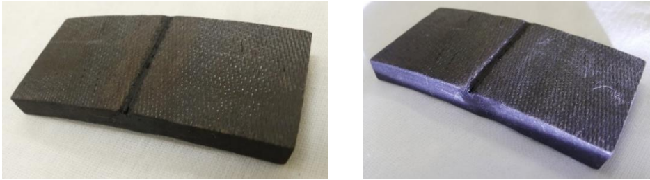
Fig. 4. Appearance of fiberglass samples with folds.
