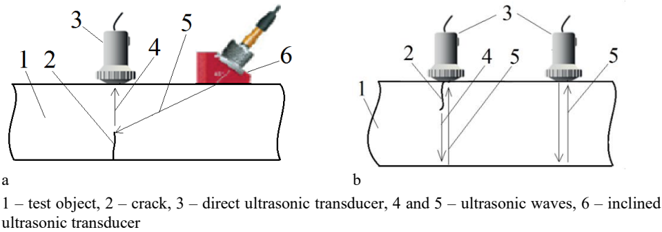
Fig. 3. Defect height measurement using first-class diffraction of ultrasonic waves (a) and a decrease in the amplitude of the diffracted wave (b).
