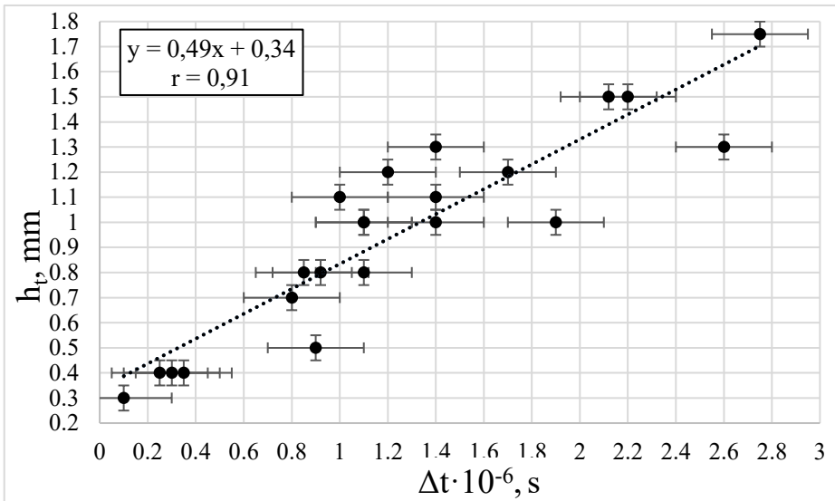
Fig. 11. Dependence of the increase in the propagation time of ultrasonic waves \Delta t on the fold on the depth of the fold h_t .
