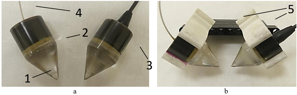
1 – conical waveguide, 2 – piezoelectric element, 3 – damper, 4 – radio frequency cable, 5 – transducer fixation mechanism with the possibility of changing the input angle
