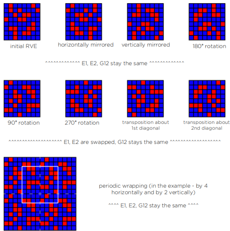
Fig. 3. The new RVEs and associated homogenised elastic properties obtained using the data augmentation scheme on an initial RVE. (2D case example. 3D case is analogous). In theory, this data augmentation scheme allows to increase the amount of samples in the training set from 8000 to 568000 (71 times more) in the 2D case, and from 800 to 424000 (530 times more) in the 3D case. However in the 3D case, we eventually used only a partial augmentation scheme, where we skipped one in every two domains when iterating through the RVE’s domains in a single direction. This was done to prevent too many very similar RVEs with identical associated properties from appearing in the new dataset, making it much less diverse. Indeed, the proportion of new and a priori less similar RVEs generated from other geometric transformations (which contributes 18 times more samples) could become too insignificant compared to those generated from periodic wrapping (which contributes 511 times more samples in the full version, and 45 times more in the partial version). With the
