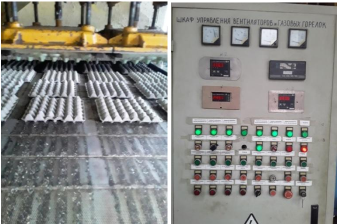
Fig. 4. Beston vacuum paper casting equipment ("Compiled by the authors").
