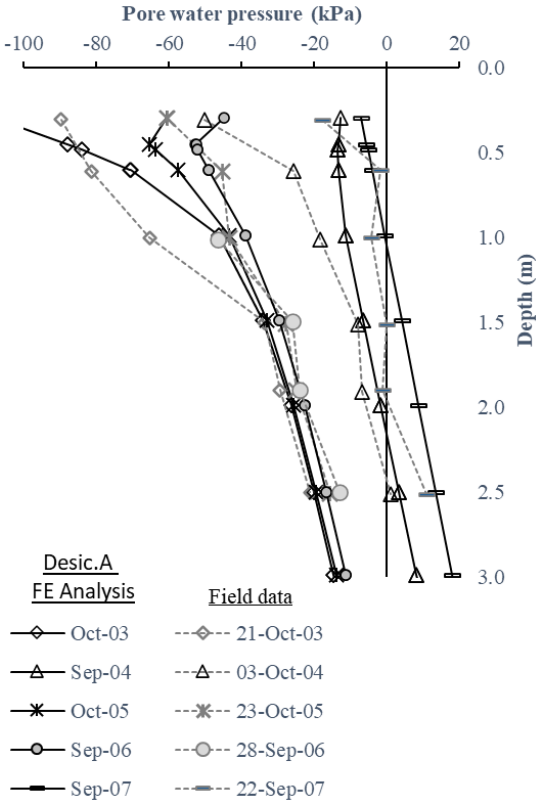
Fig. 9. Desic.A slope analysis results in comparison to field data by Smethurst et al. (2012)
