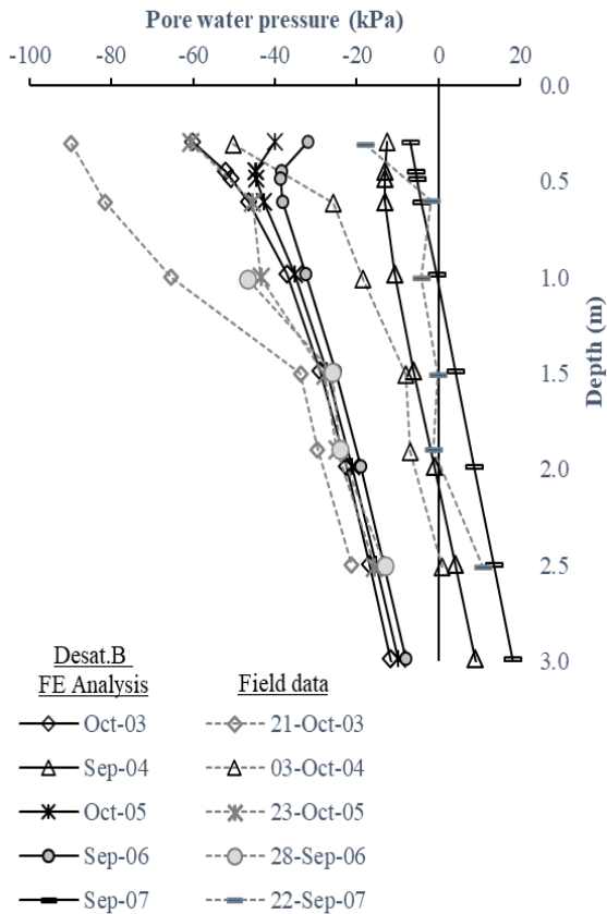
Fig. 8. Desat.B slope analysis results in comparison to field data by Smethurst et al. (2012)
