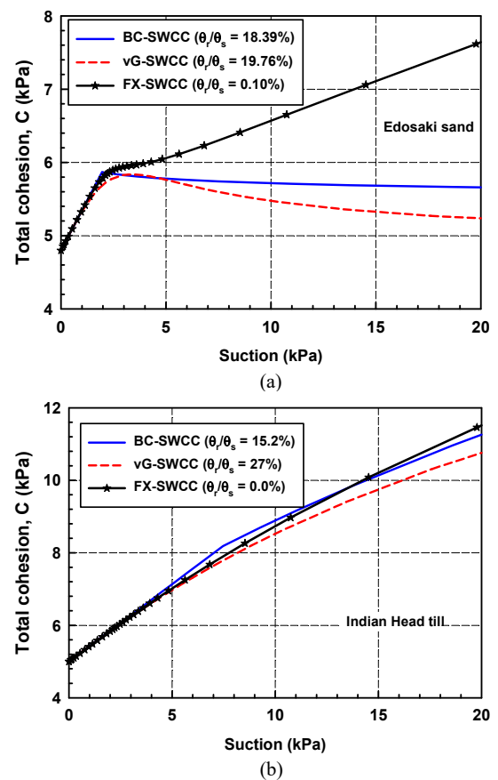
Figure 4. Variation of total cohesion with respect to suction obtained with three different SWCC fit models and Eq. (4): (a) ES and (b) IHT.
