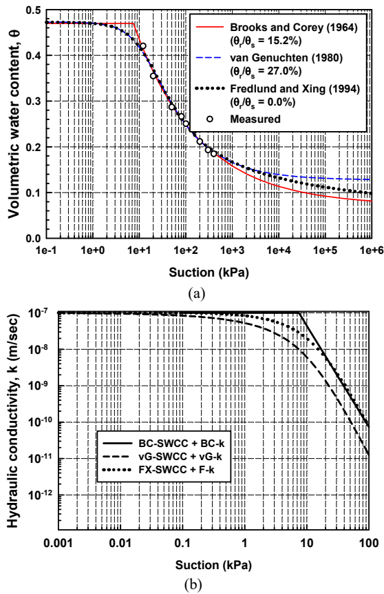
Figure 3. Indian Head till: (a) SWCCs and (b) hydraulic conductivity functions.
