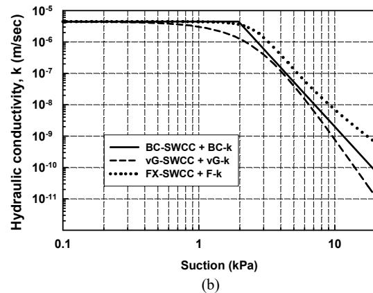
Figure 2. Edosaki sand: (a) SWCCs and (b) hydraulic conductivity functions.
