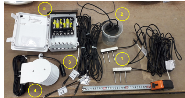
Fig. 1. Sensors installed in the mudbricks and mudbrick walls along with the logger used (explanation according to numbers in the text).
