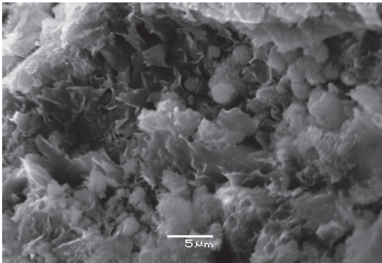
Fig. 14. SEM image of Aggeria bentonite. Opal-CT lepispheres are hosted in between the montmorillonite sheet-like crystals.
