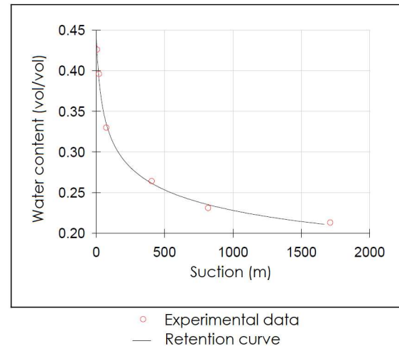
Fig.8. Retention curve of sample 3 (1 year)
