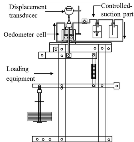
Fig. 2. Experimental setup for suction-controlled oedometer tests.
