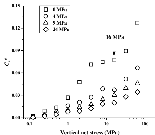
Fig. 8. C_c^* versus vertical net stress.
