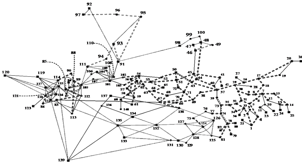
Fig. 2. NPCC 140-bus power system.
