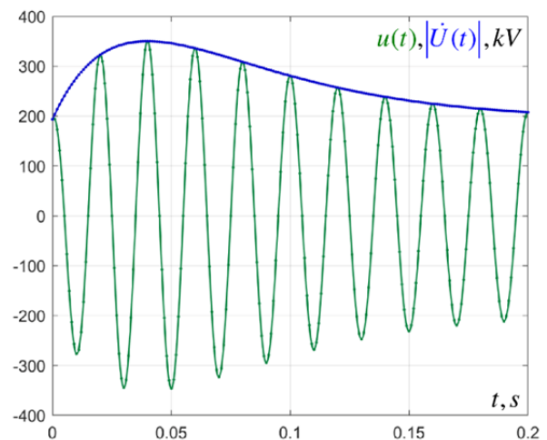
Fig. 5. Instantaneous voltage values and total voltage synchrophasor module.
