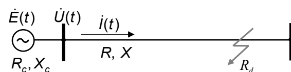
Fig. 1. Equivalent circuit.
