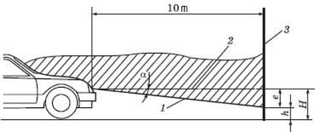
Fig. 2. Arrangement diagram of the vehicle's headlight relative to the measuring screen: 1 – cutoff line; 2 – axis of reference; 3 - matte screen.
