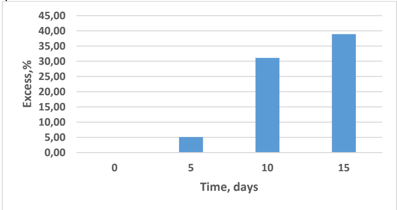
Fig. 1. Excess of Ni bioleaching with 1% persulfate over bioleaching without persulfate from silicate ore by A. ferrooxidans VKM B-3655, %.
