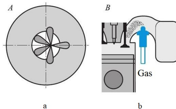
Fig. 2. The system for supplying oil diesel fuel to the cylinder of the D-245 gas diesel engine, which forms jets of atomized fuel (a), and the system for supplying hydrogen to the engine intake system (b).
