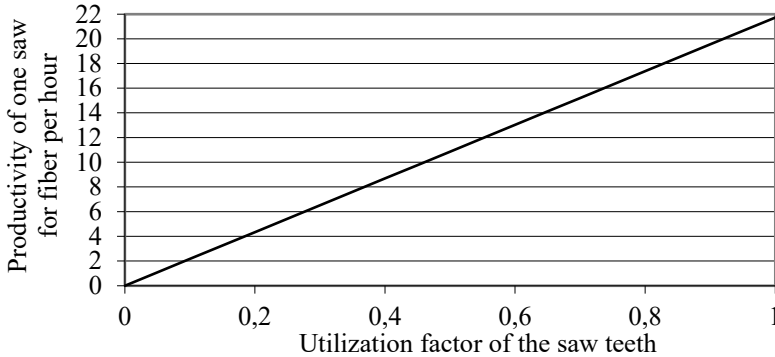
Fig. 1. Change in the productivity of one saw for fiber in kg/h.
