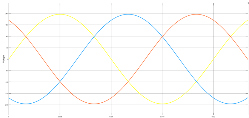
Fig. 10. Input voltage of the three-phase full converter
