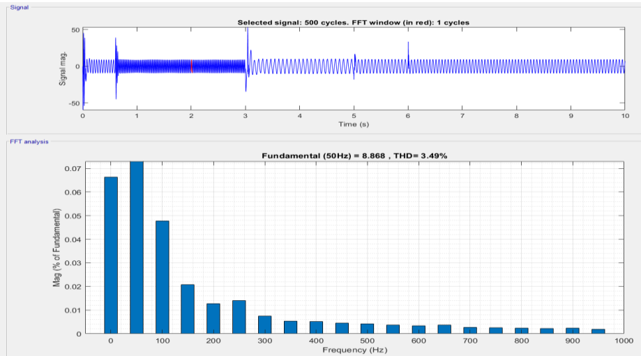
Fig. 21. THD value when PID controller is used
