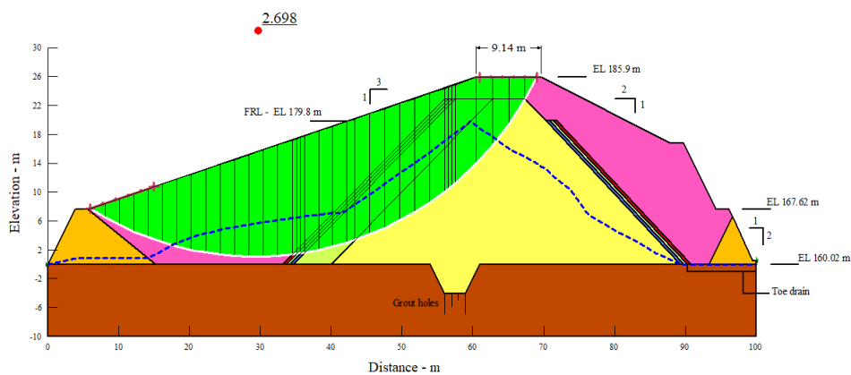
Fig. 11: Upstream Slope Stability after instantaneous drawdown for 5 days
