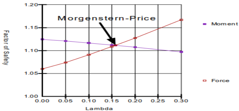
Fig. 3: MP safety factor for half-sine function
