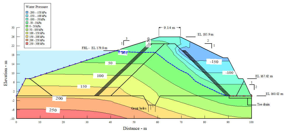
Fig. 7: Pore Water Pressure distribution in seepage flow The pore water pressure inside the dam through steady state seepage is displayed on figure 7. Downstream and upstream slope stability analyzed by using SLOPE/W shown in Fig. 8 and Fig. 9 respectively.
