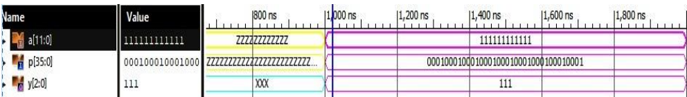
Fig. 5. 36-bit matrix multiplier simulation result.
