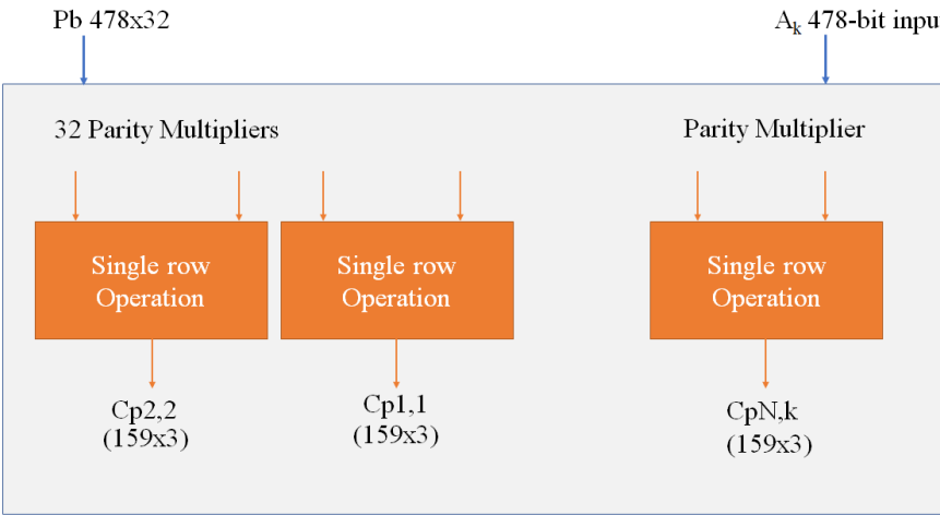
Fig. 3. Block diagram of 478-bit matrix multiplier.
