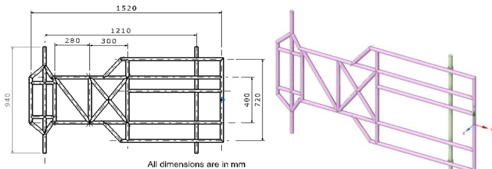
Fig. 1. Drawing views of 3D model frame chassis.
