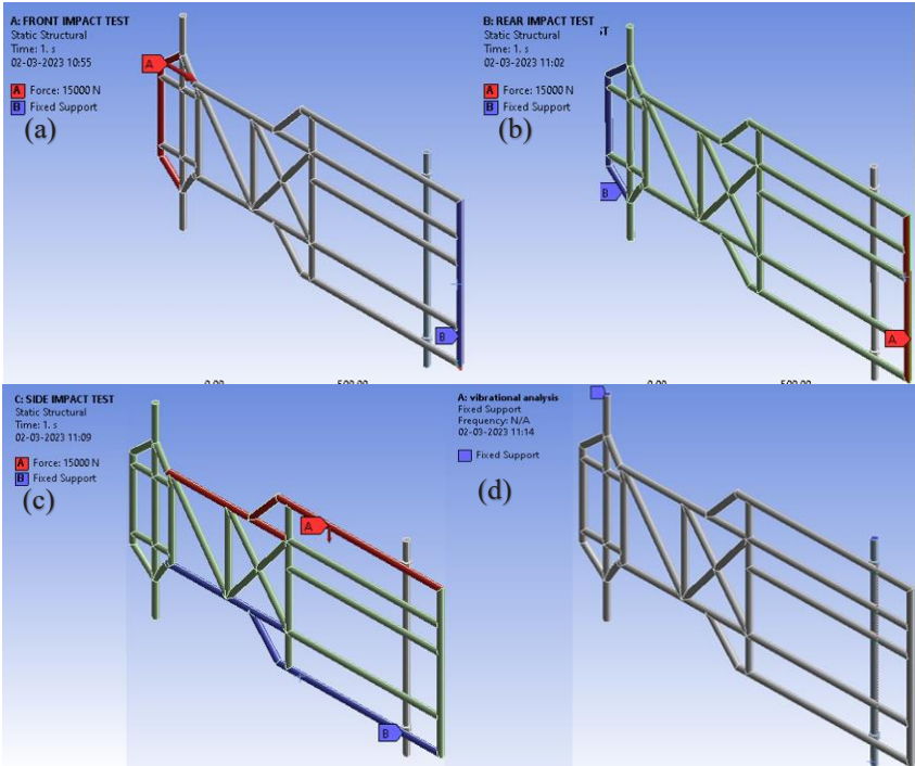
Fig. 2 Static structural and Modal analysis boundary conditions (a) Front collision test (b) Rear collision test (c) Side collision test (d) Vibrational test.
