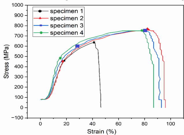
Fig. 9. Stress strain graph for the specimens
