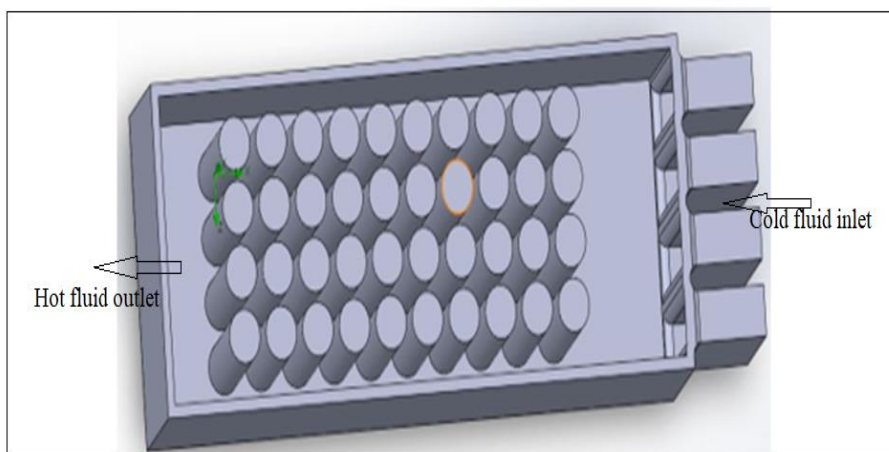
Fig. 3. Geometry 3 for Air and Direct Liquid cooling model
