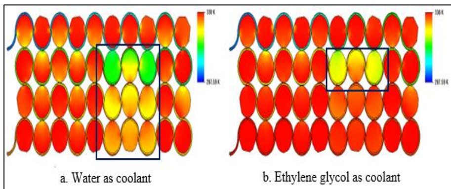
Fig. 5. Horizontal temperature distribution with Channel cooling (a) Water coolant (b) Ethylene glycol coolant
