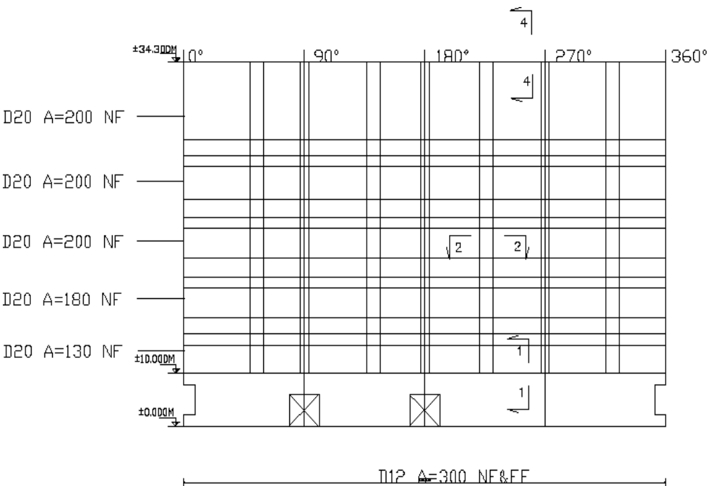
Fig.3: Reinforcement details for Top wall
