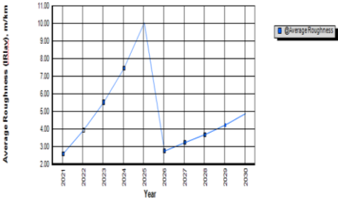
Figure. 9. Prediction data of GM
