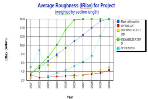
Figure. 13. Average roughness overall route HDM-4
