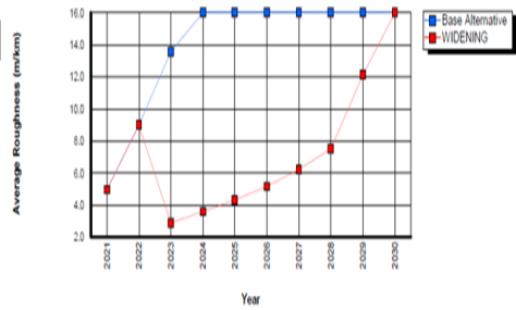
Figure. 11. Average Roughness of KD
