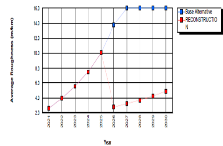
Figure. 8. Average Roughness of GM Route
