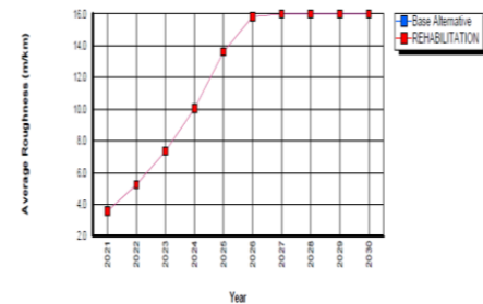
Figure.12. Average Roughness of BD
