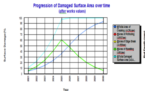
Figure. 14 Overall surface in HDM-4
