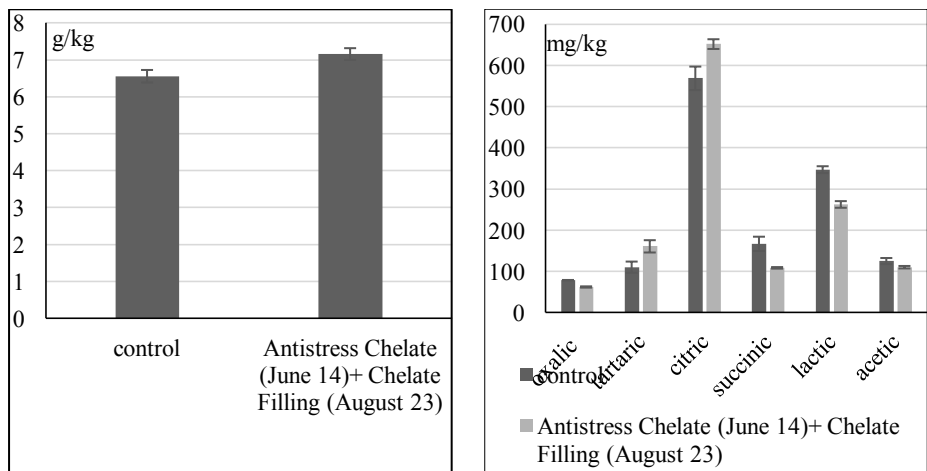
Fig. 2. The content of organic acids in apple fruits when treated with agrochemicals: a) the content of malic acid; b) the content of other organic acids.
