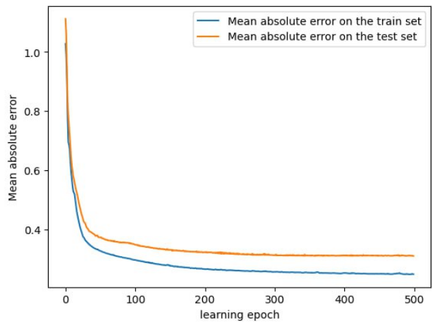
Fig. 2. Neural network training.
