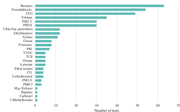
Fig. 3. The number of times that pollutants tested in review studies
