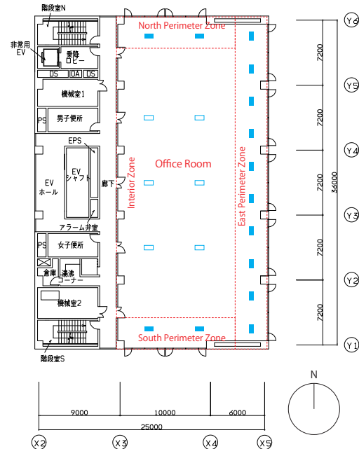
Fig. 1. Standard floor plan
