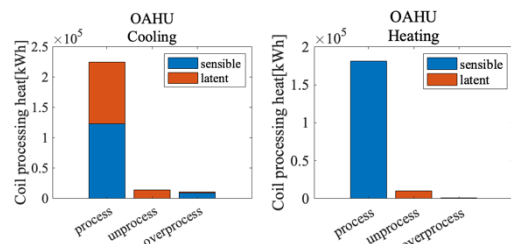
Fig. 12. Coil processing heat (low-level case)
