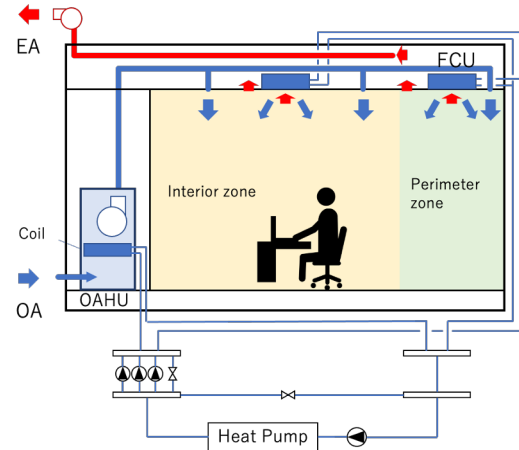
Fig. 3. System overview (OAHU system)
