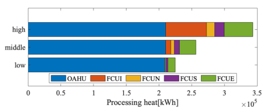
Fig. 15. OAHU system processing heat during cooling season
