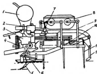
1 – reservoir; 2 – filter; 3 – pump; 4 – conical reducer; 5 – furrow openers; 6 – support slide; 7 – valve dispenser; 8 – reducer; 9 – parallelogram mechanism; 10 – cross beam; 11 – needles; 12 – spools
