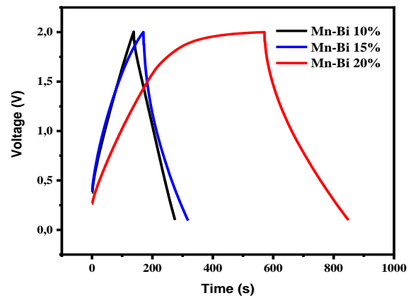
Fig. 4 Curves (a) charge-discharge of AC-Mn 2 O 3 -BiPO 4 film electrodes with variations of 10, 15, and 20% and (b) charge-discharge variations of 20% for 10 cycles
