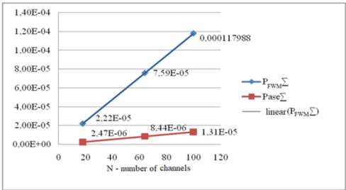
Fig. 5. Dependence of P FWMΣ and P ASEΣ on the number of channels
