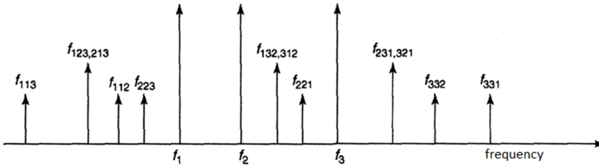
Fig. 2. Mixture of products generated thanks to the FWM for 3 optical signals [1].
