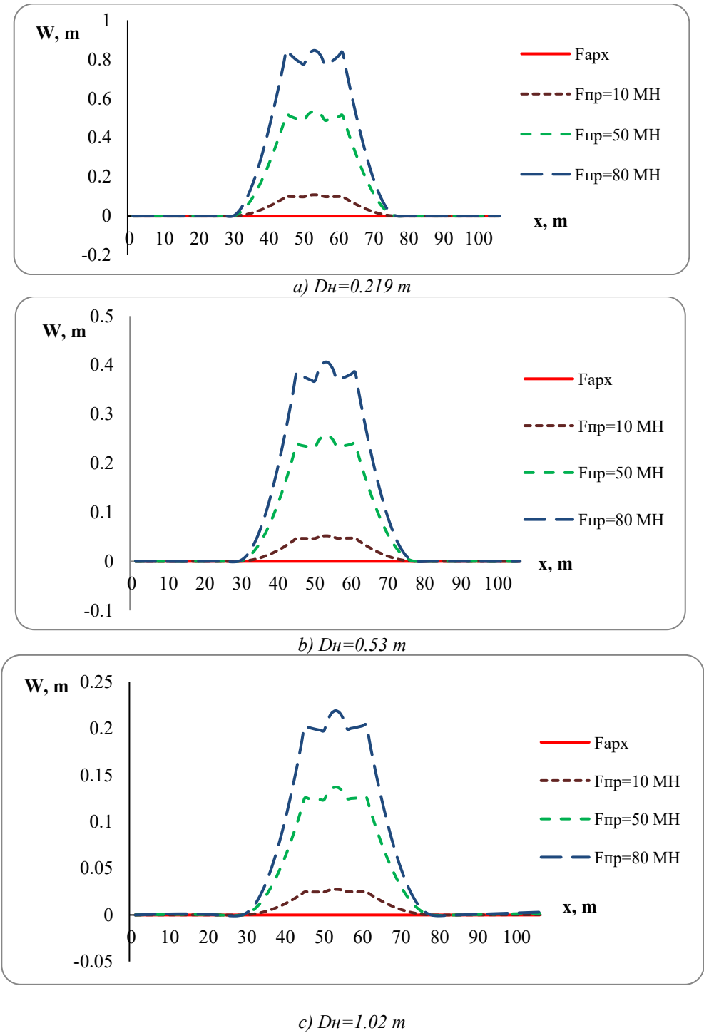
Fig. 1. Buckling of the buried gas pipeline with a \Pi -shaped part along axis Z with a configuration equal to 5 m: F_{apx}=579.3\text{ H} ; F_{np}=(10\text{ MH}, 50\text{ MH}, 80\text{ MH}) ; liquefied area 40 m.
