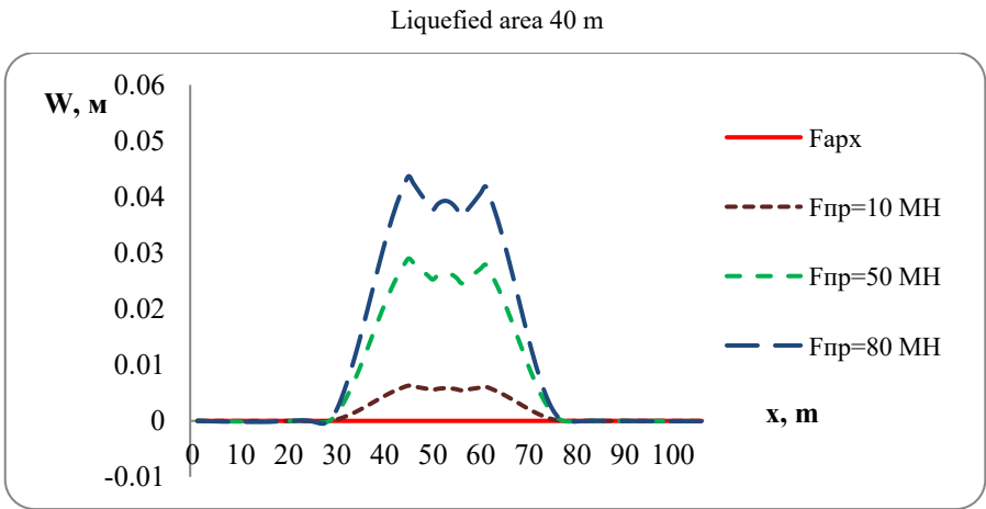
a) \Pi -shaped part of the pipeline along axis Y with a configuration equal to 5 m
