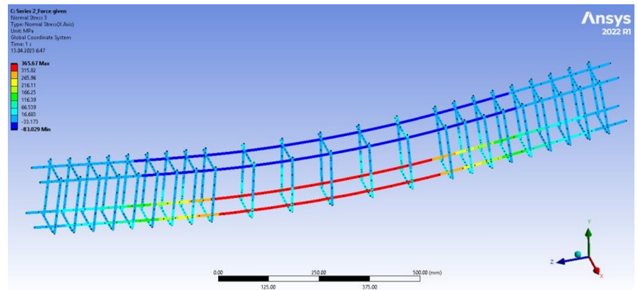
Fig. 6. Variation ranges of rebar stresses for Series 2, MPa
