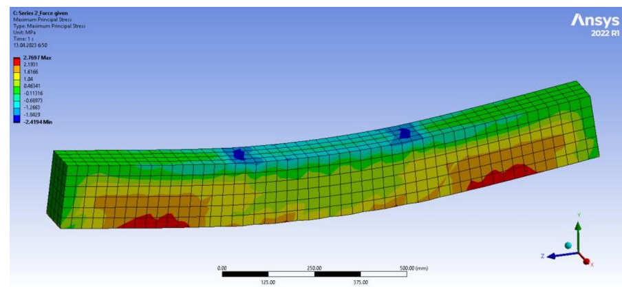
Fig. 7. Variation ranges of concrete stresses for Series 2, MPa
