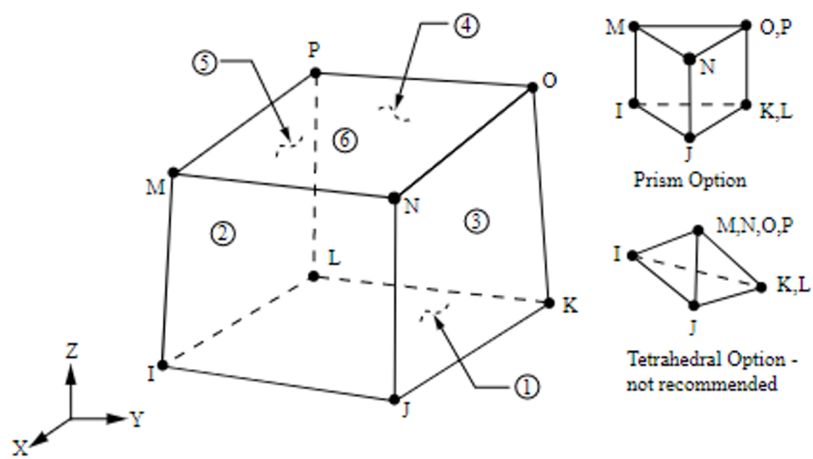
Fig. 3. CPT215 Structural Solid Geometry
