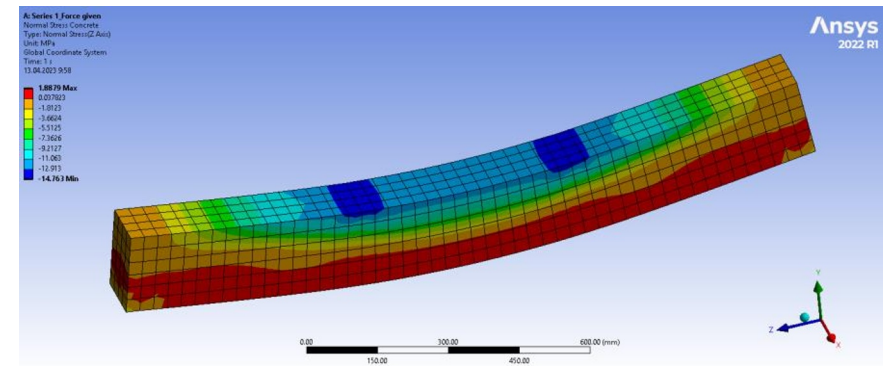
Fig. 5. Variation ranges of concrete stresses for Series 1, MPa
