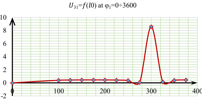
Fig. 3. Graph of the change in gear ratio U_{31} from the distance l_0 .
