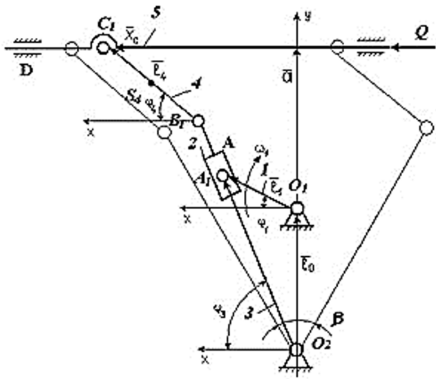
Fig. 1. Cross planer mechanism
