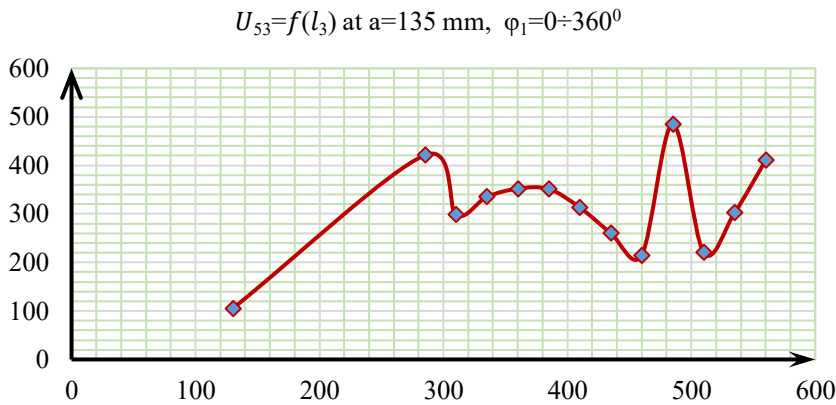
Fig. 7. Graph of the change in gear ratio U_{43} (link - connecting rod) on the length of the link.
