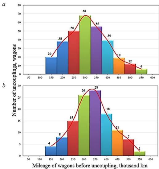
Fig. 4. Dependence of the number of uncoupled gondola wagons of the model 12-9853 on the fault of the thin rib (a) and the shelled tread of the wheel (b) on the mileage of the wagons before uncoupling on CR-2
