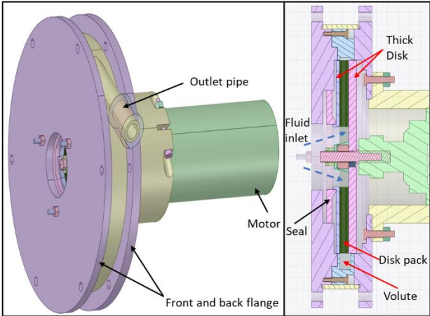
Figure 2: Reversible Tesla machine: 3D and cross-sectional view.
